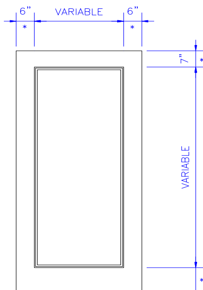
TYPE "FG"
