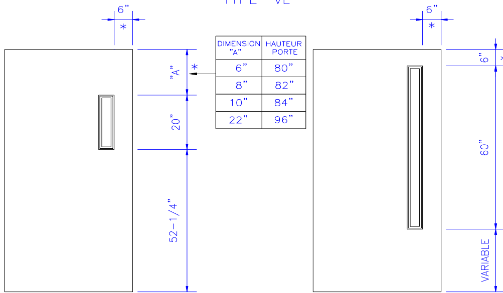
TYPE "NL"
