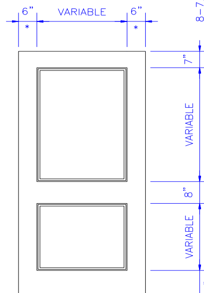
TYPE "FGWR"
