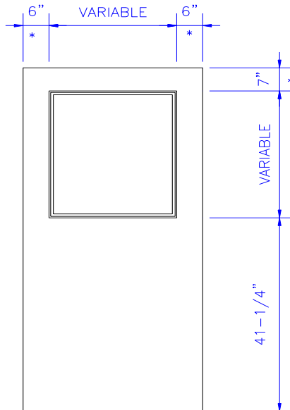
TYPE "HG"
