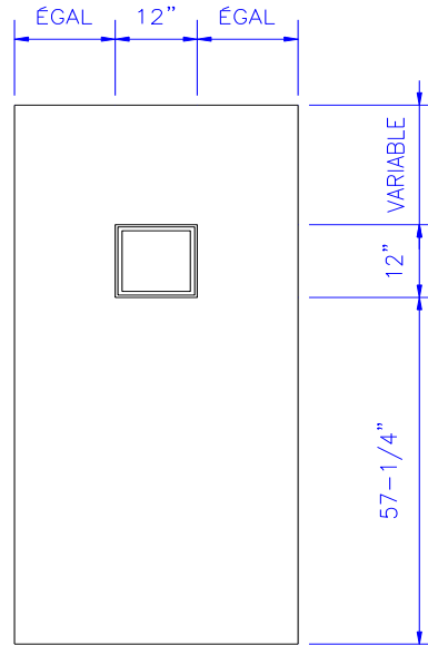
TYPE "VL"
